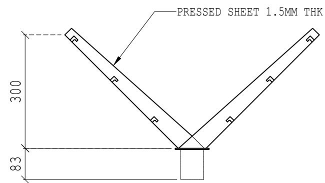
1 LIGHT EXTENSION ARM Scale: NTS
